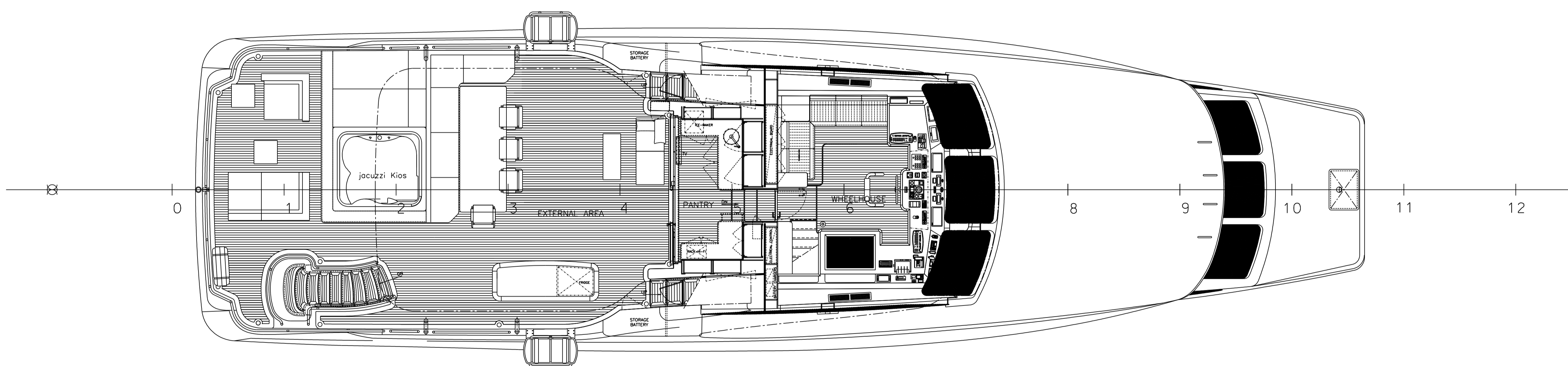
UPPER DECK
