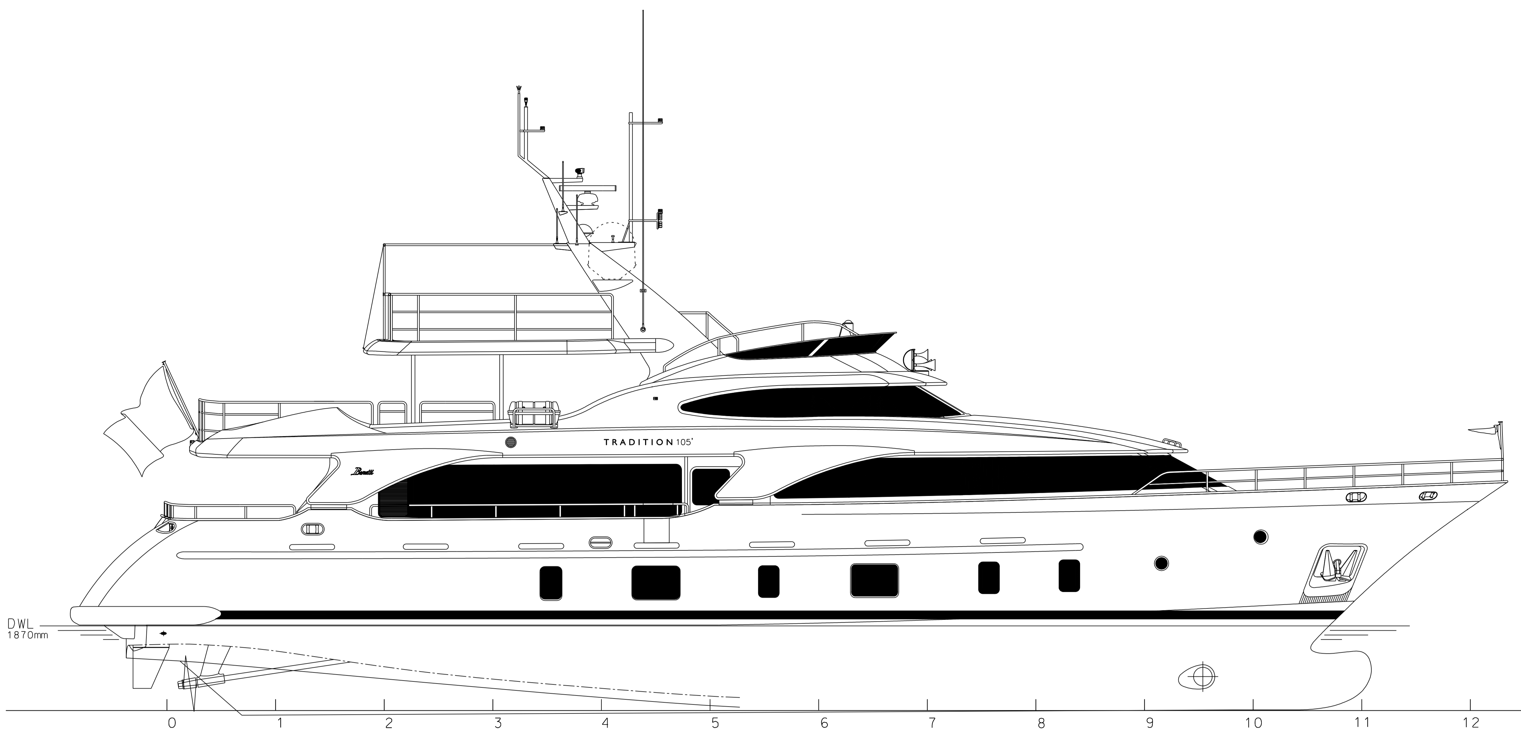
PROFILE
