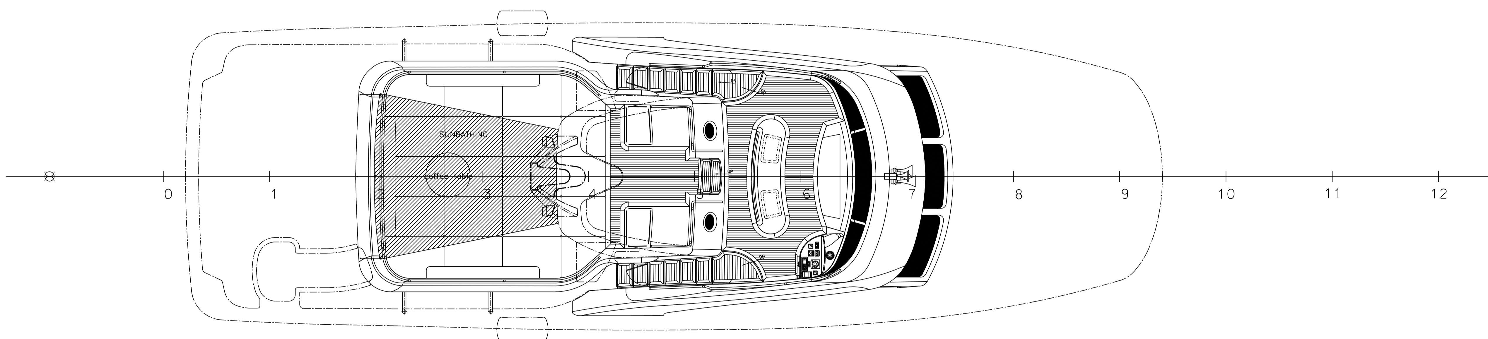
FLY BRIDGE & SUN DECK
